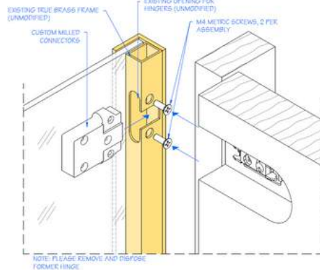
CUSTOM MILLED CONNECTORS x 20 (+2 spares)
